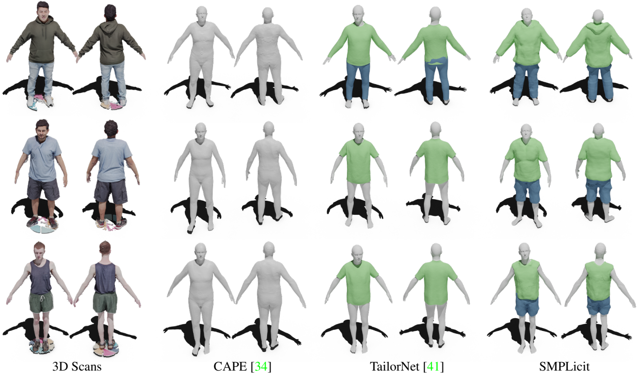
Figure 4: Fitting SMPLicit to 3D Scans of the Sizer Dataset [57] . All three models achieve fitting results of approximately 1 mm of error. However, SMPLicit does this using a single model that can represent varying clothing topologies. For instance, it can model either hoodies (top row) and tank tops (third row) or long and short pants.
